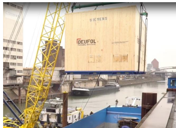
Picture: Loading of a Siemens crate, designed and packed by Deufol with almost 300 tons weight. (Photo: Deufol)
